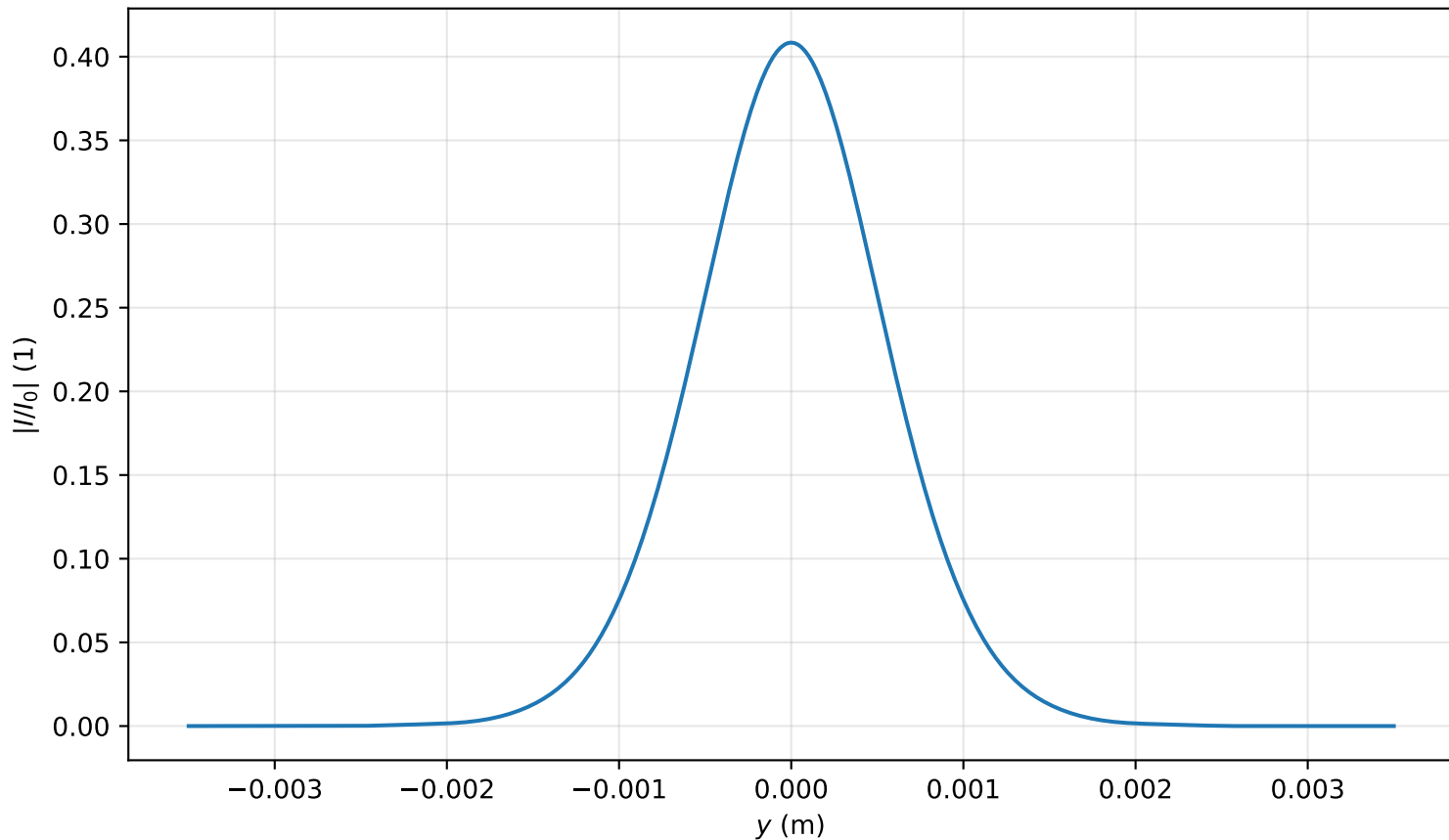
Intensity profile I(x=0, y, z=3.423)/I_0 , P_{in}=0.4P_{cr} , artificial time
